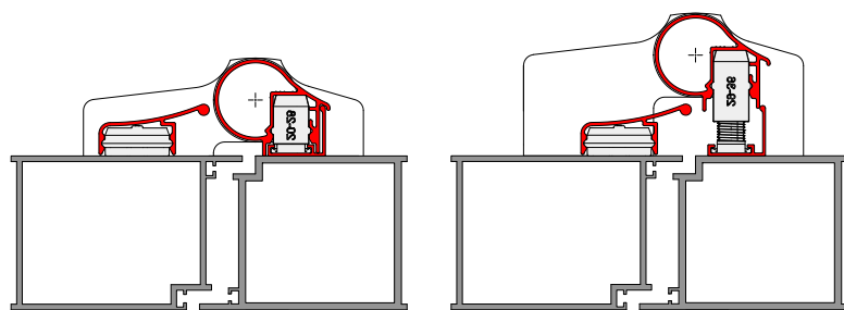
BA-28+ with different surface mounted hinges
