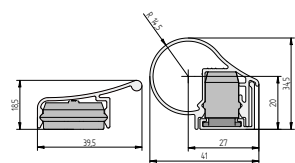
Profile door leaf
